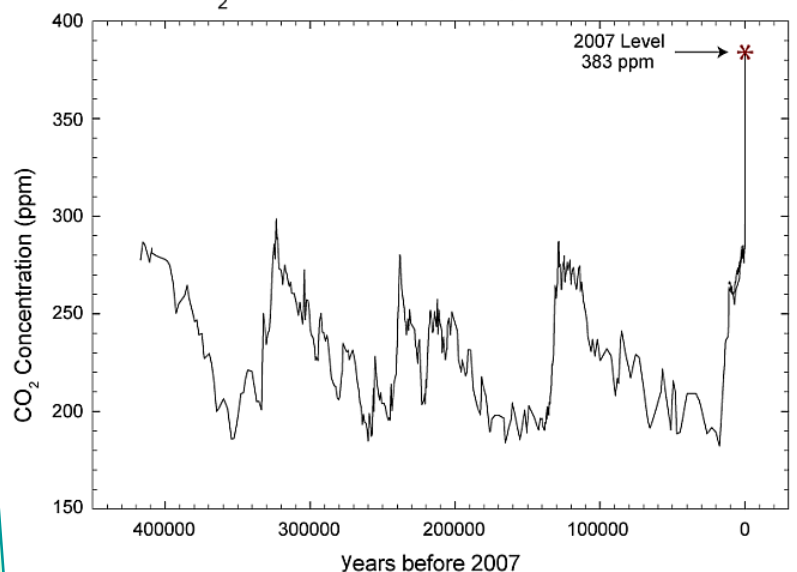
CO 2 Over Past 420 Thousand Years
